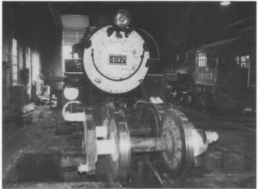
Thanks to the efforts of Friends Phil McDonald, Jerry Sahnd, Gerald Blea, Roger Briggs, and Mark Yates, freshly painted locomotive 497 sits in the Chama enginehouse awaiting the installation of the drivers—two sets are in the foreground. The team spray painted the locomotive in the Chama enginehouse on February 26, 2000. (Photo by Tom Cardin.)
